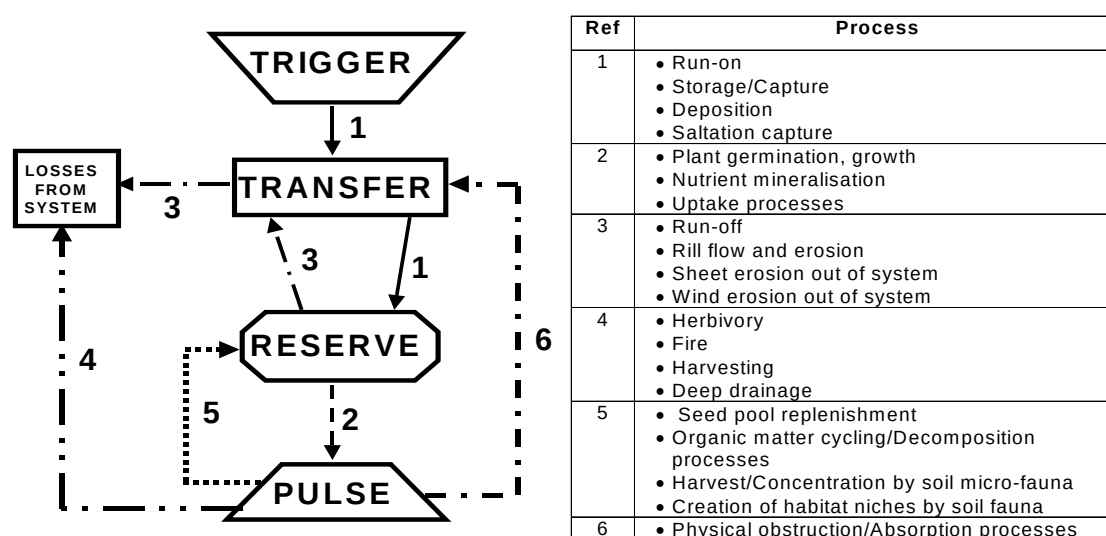
Figure 5. The conceptual framework representing sequences of ecosystem processes and feedback loops. The table lists some of the processes operating at different locations in the framework.
