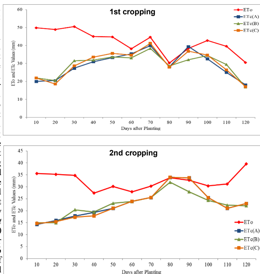
Figure 4. Actual and reference crop evapotranspiration of IPB Var13 corn variety for both cropping seasons.
