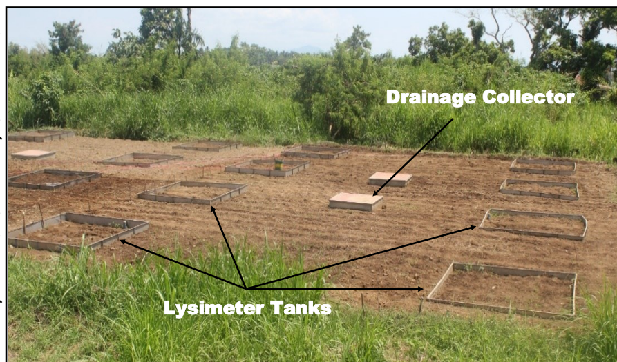
Figure 2. Lysimeter Setup.
