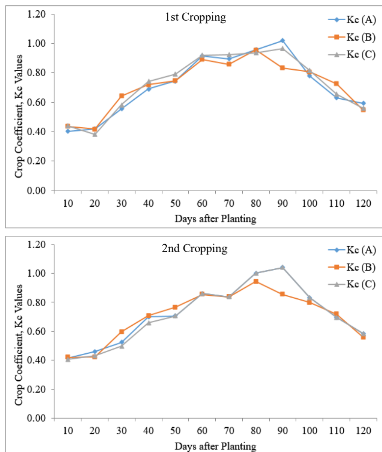
Figure 5. Decadal values of crop coefficient, Kc for both cropping seasons of IPB Var13 corn variety.
