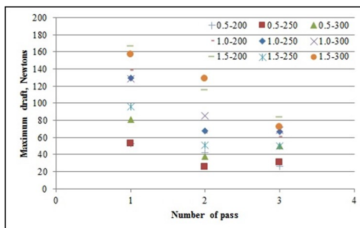
Figure 2. Maximum draft with 0° lug angle at varying forward (0.5, 1.0 and 1.5 km h -1 ) and shaft speeds (200, 250 and 300 rev min -1 ).
