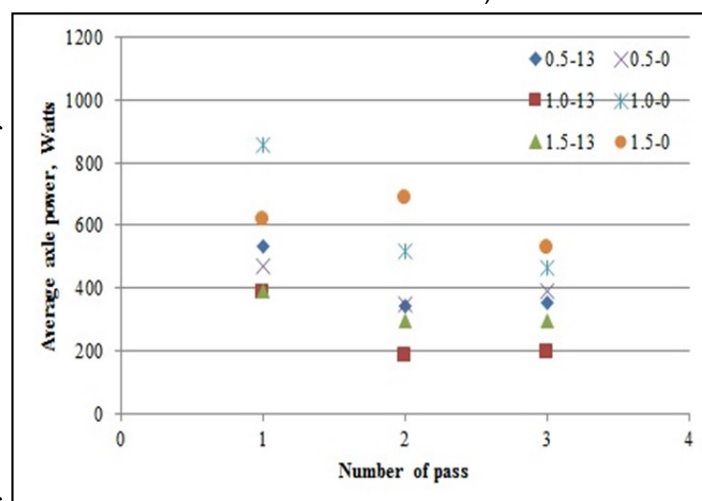
Figure 3. Average axle power with different lug angle (0° and 13°), forward speed (0.5, 1.0 and 1.5 km h -1 ) and 200 rev min -1 shaft speed.
