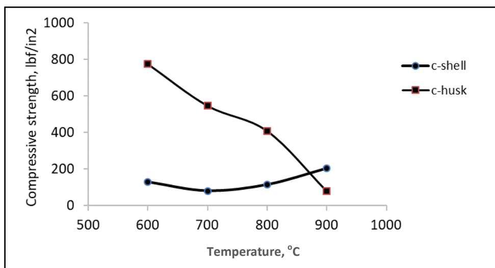
Figure 1. Compressive strength curve of c-husk and c-shell ash pellets heated at varying temperatures.
