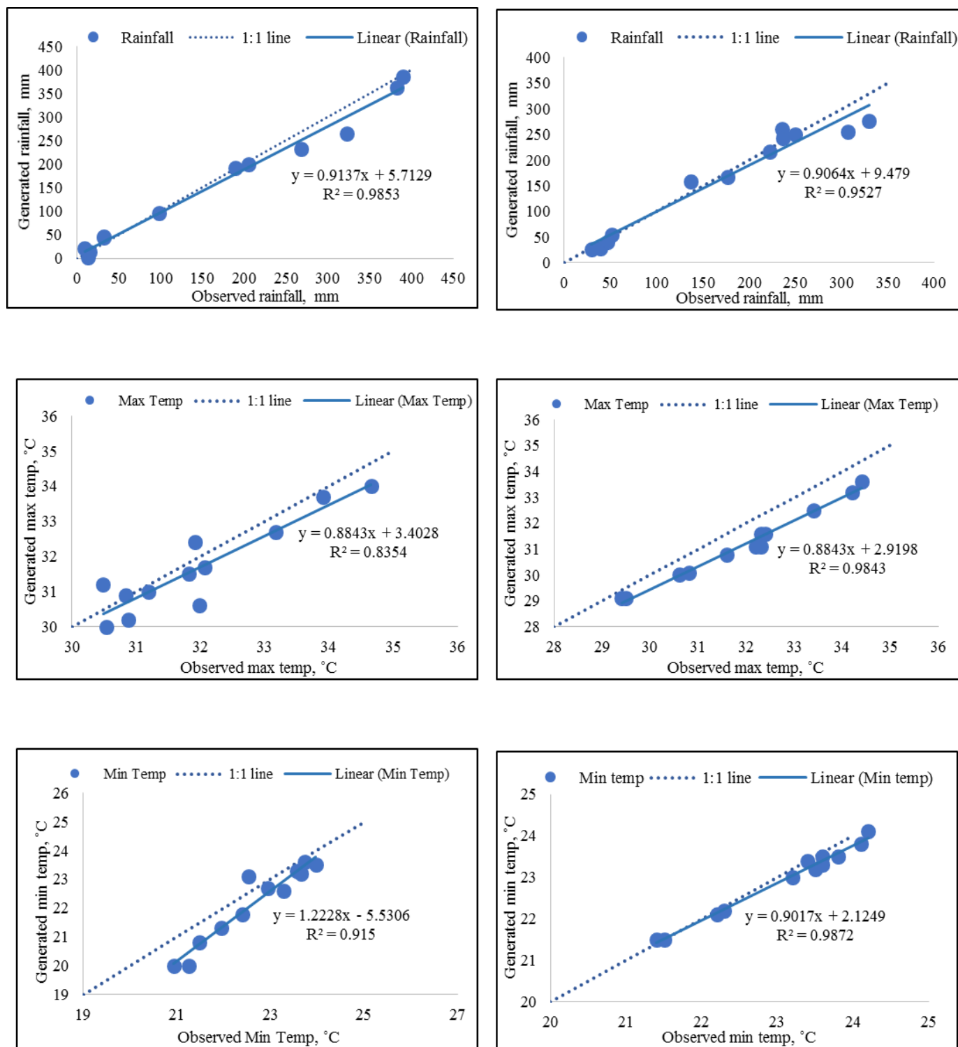
Figure 1. Linear regression analysis on rainfall, maximum temperature, and minimum temperature in (a) Muñoz, Nueva Ecija and (b) Los Baños, Laguna.
