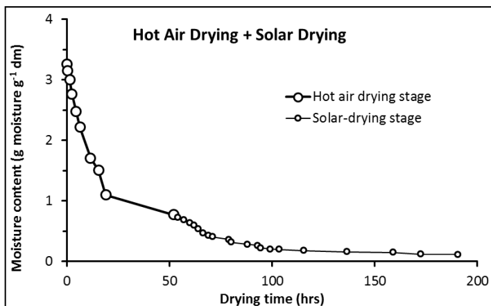
Figure 3. Drying curve of sea cucumber ( H. scabra ) samples during Treatment II
