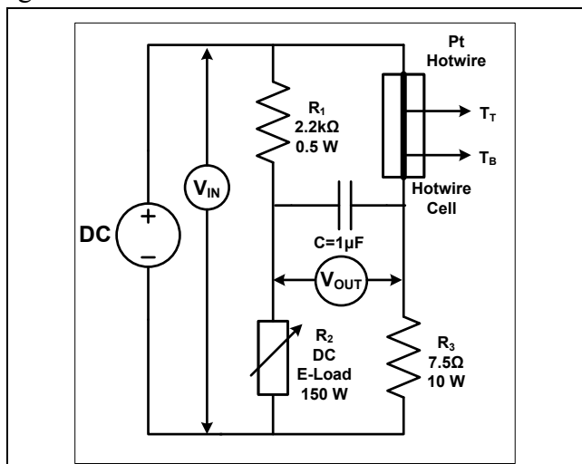
Figure 3. Schematic diagram of the thermal conductivity measurement apparatus.
