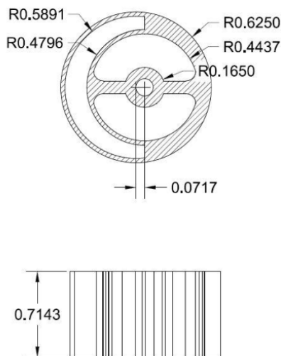
Figure 2. Alignment ring dimensions
