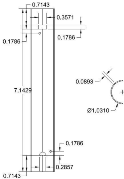
Figure 1. Half-pipe dimensions
